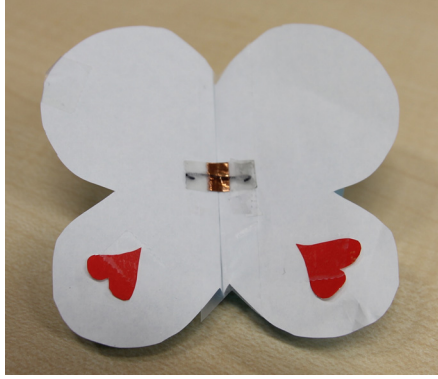
Figure 12: Animated paper butterfly. There is a SMA strip on the center of the butterfly. When the SMA is heated, it shrinks and pulls both wings together, creating a flapping motion.
