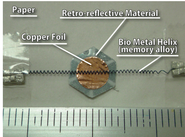
Figure 7: The marker for laser system. Our system consists of three key components which are affixed to the paper: SMA(Bio Metal Helix) which serves as an actuator, Retro-reflective material which works as a marker, and Copper foil which we use as thermal absorber.
