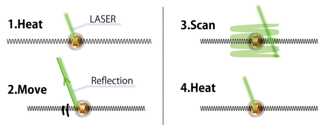
Figure 11: Tracking sequence. 1: Laser heats the center of the marker where the copper foil is affixed. 2: Laser hits the retro-reflective material and the light is reflected back to the photo sensor. 3: Sensor detects the movement of the marker and the laser scans again to find the new center. 4: Laser heats the copper again.
