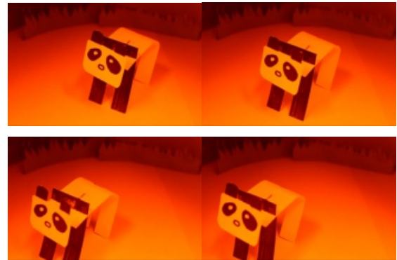
Figure 3: Walking paper toy: This panda paper craft walks when the SMA located above the forefeet is heated by the laser.
