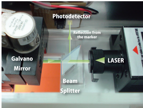
Figure 5: The position of Laser, Galvano mirror, Beam splitter and Photodetector to prevent any eye damage from the laser beams, we have built a special box that is covered by aluminum to prevent laser emission. This box has a window made of acrylic which acts as a laser filter, allowing the user to perfectly see the inside without any retinal harm.
