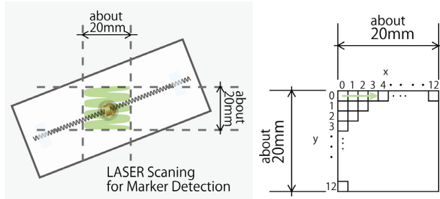
Figure 8: Tracking area. The laser scans the 20[mm] x 20 [mm] square to find the center of the marker by dividing it into 169 areas.
