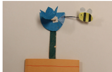
Figure 13: spinning movement. The bee is connected to the flower by a short SMA helix. When the laser heats the SMA, the SMA shrinks in a spiral motion, so that the bee spins toward the flower.
