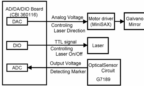
Figure 4: Block diagram of animated paper's control system. The AD/DA/DIO board controls the motor driver and laser, and receives the data from the optical sensor circuit.
