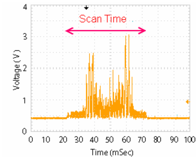
Figure 9: Marker and tracking area (top left), Laser tracking the marker's center point (top right), Output waveform of photo sensing circuit (bottom)
