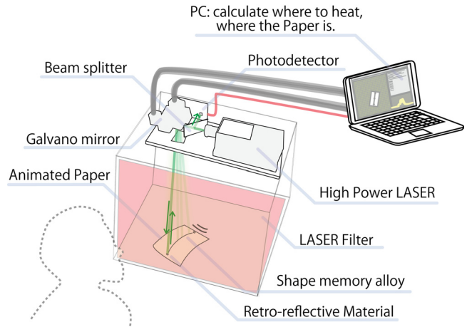
Figure 6: System overview. The metal box has a laser filter with a protected opening at the top through which the laser passes through to control the paper figure in the box.
