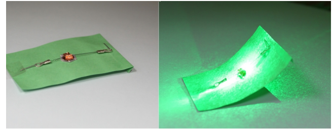
Figure 10: Animated paper module (left), bending movement (right). The maximum angle of the bending motion is around 60 degree.
