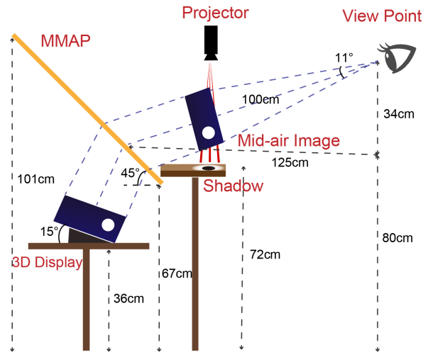
Figure 1: Optical design; a projector is used to project a shadow directly below a three-dimensional mid-air image using a 3D display.
